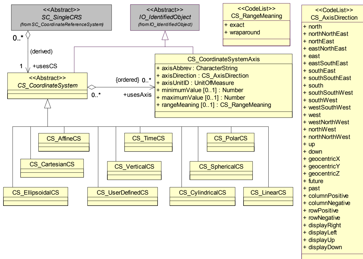
Figure 8 — CS Coordinate System package
