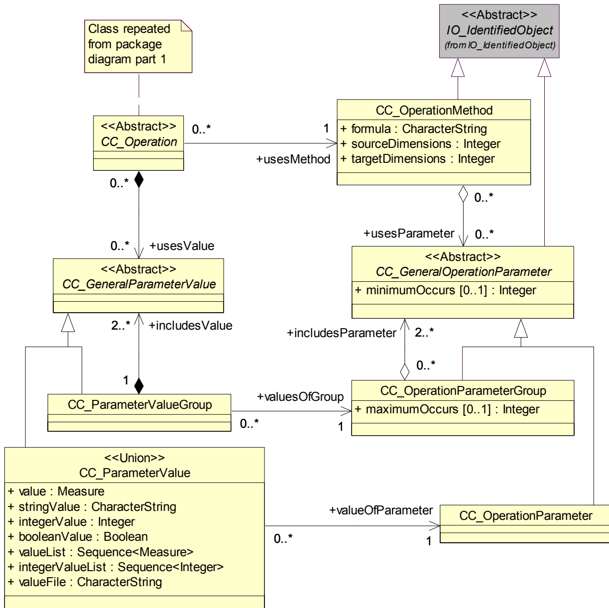
Figure 13 — CC Coordinate Operation package part 2
