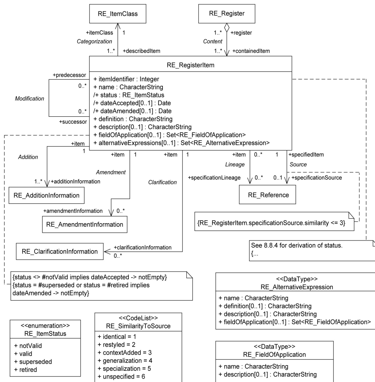
Figure 14 — RE_RegisterItem
