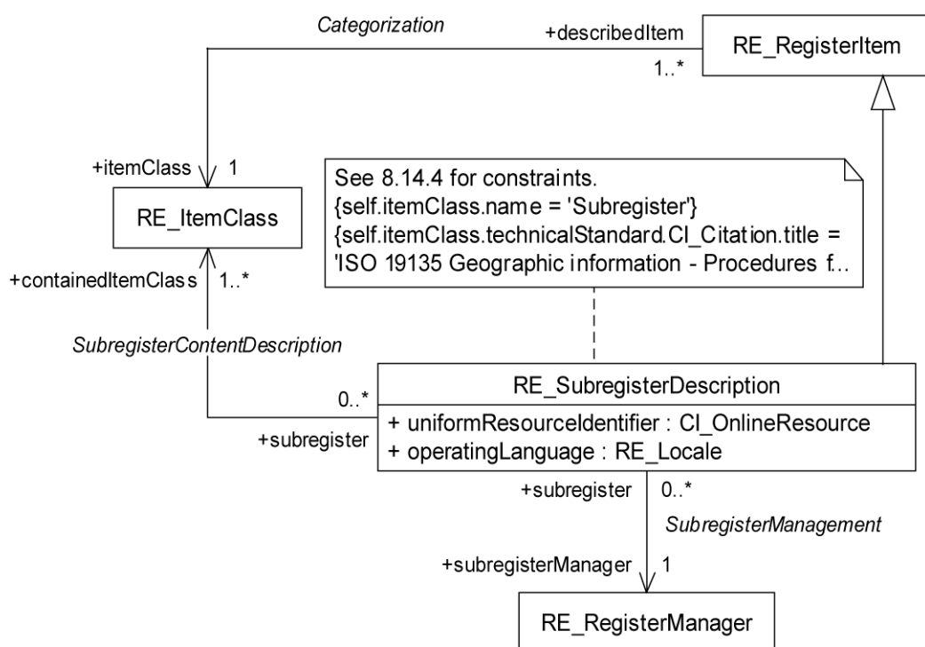
Figure 17 — RE_SubregisterDescription
