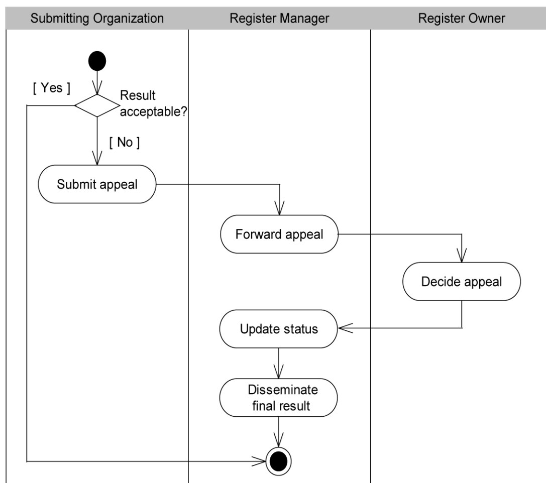
Figure 4 — Appeal process
