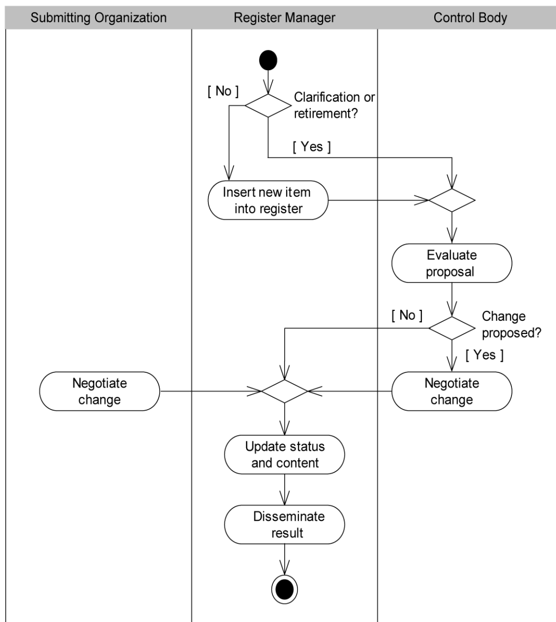
Figure 3 — Approval process
