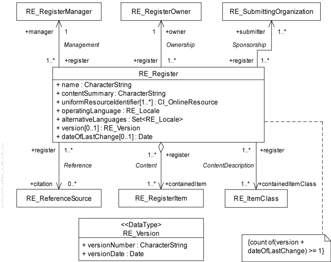
Figure 8 — RE_Register
