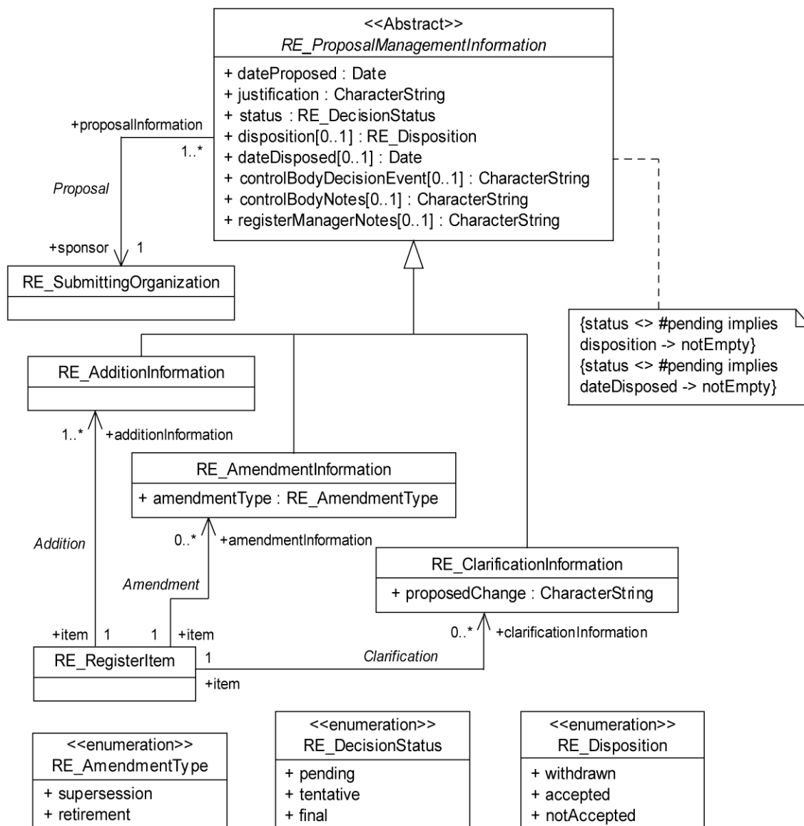
Figure 15 — RE_ProposalManagementInformation
