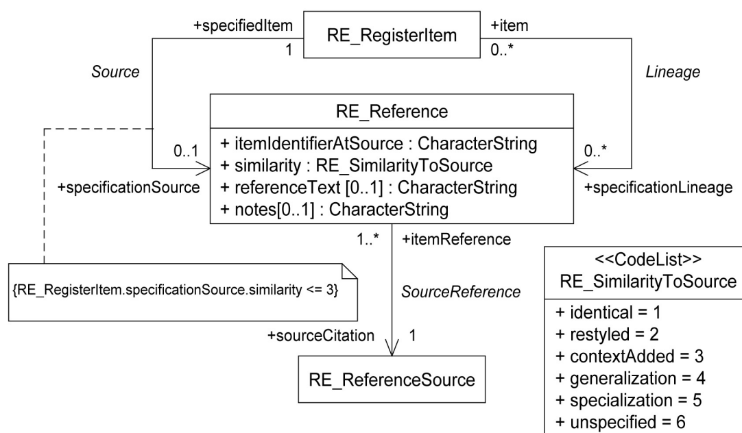
Figure 16 — RE_Reference
