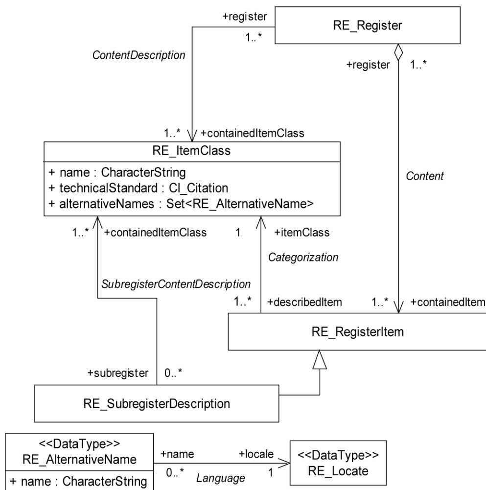
Figure 12 — RE_ItemClass
